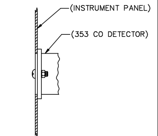
SECTION F-F
