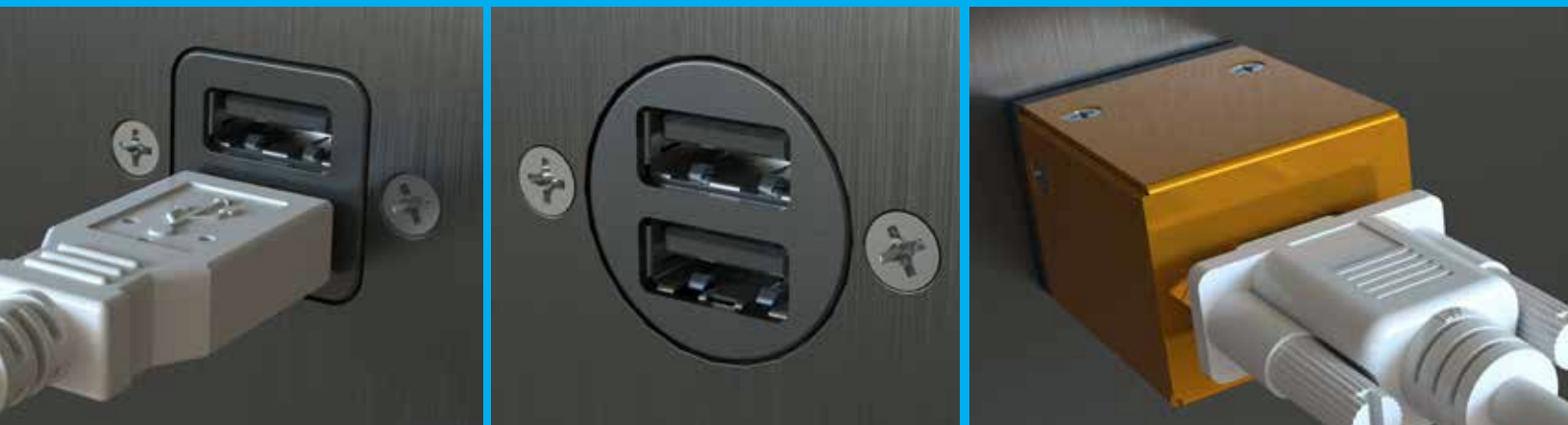
Panel mounted 250-101 installed (left), 12v socket / cigarette lighter replacement (center), and behind the panel (right)
